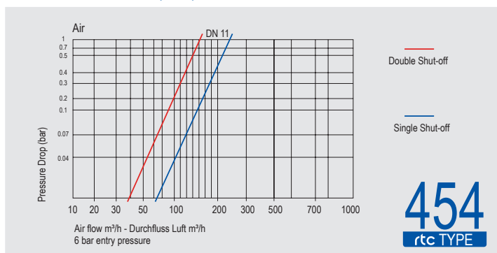
Flow Rate vs Pressure Drop Graph
